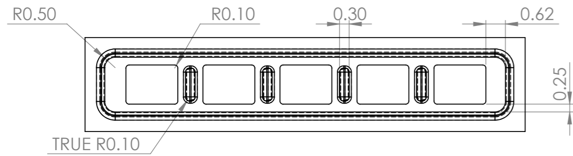
Bottom view
