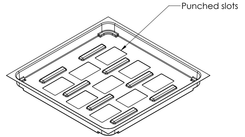
Isometric View
