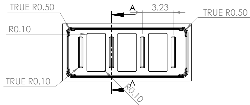
Bottom view
